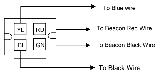
Tx3600/3820/4800 Interface Plug 3E-7808 (Looking at the front of the radio socket)
