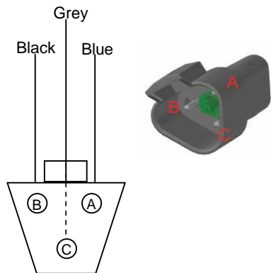
Tx3600/3820/4800 Interface Plug RCT LM-2C-129 (Looking at the front of the radio socket)
