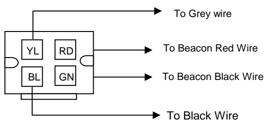
Tx3600/3820/4800 Interface Plug RCT LM-2C-129 (Looking at the front of the radio socket)
